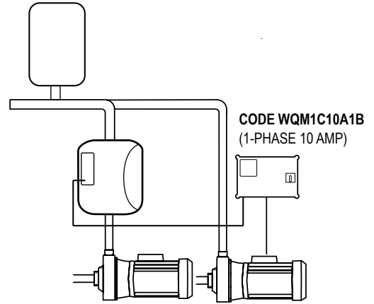
Group 1 - Boosting system with 1 pump driven by E-Power and a second pump ON/OFF piloted by E-Power through a control panel
